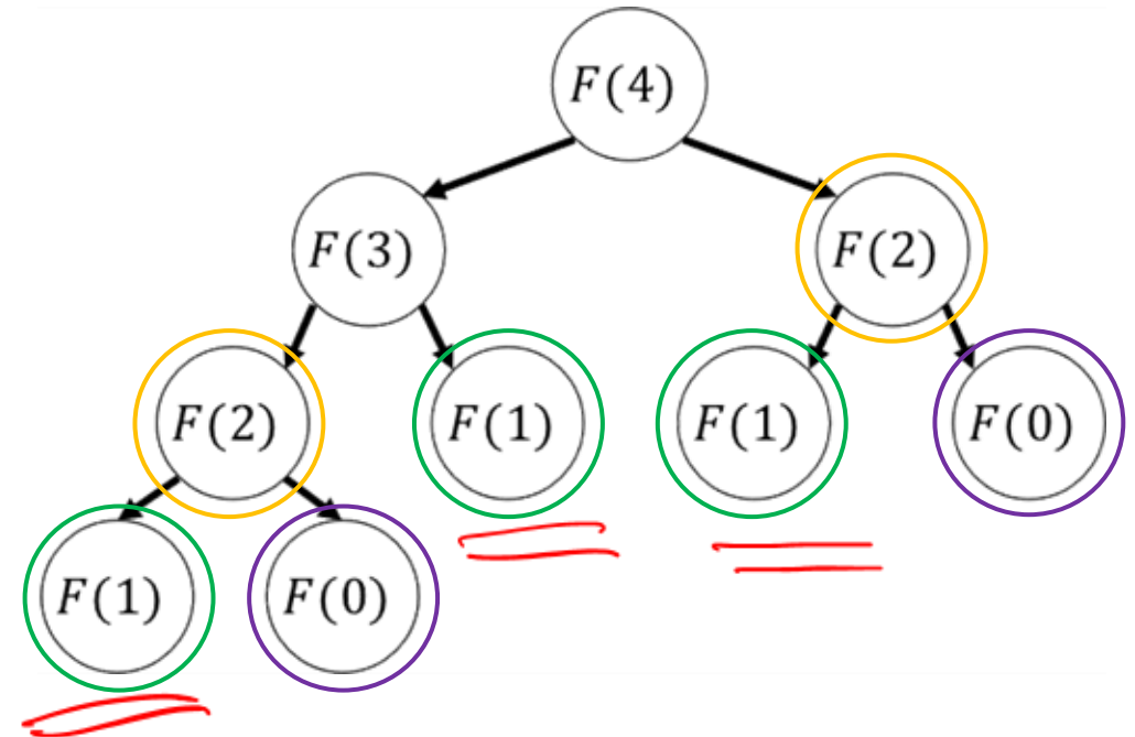
Fibonacci with re-occurring subproblems circled
